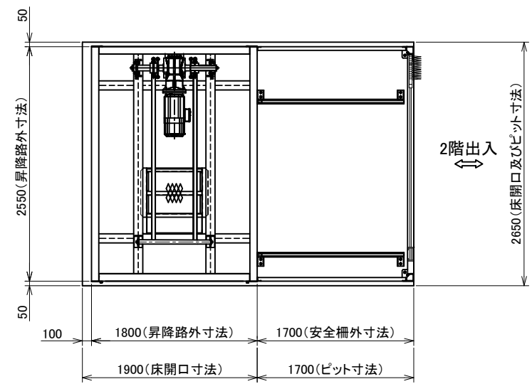
S2-S2 (2F平面)
